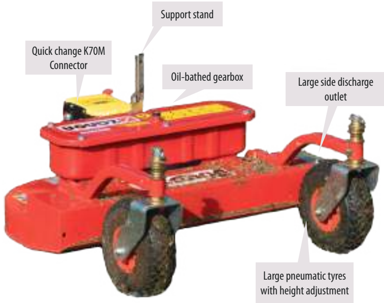
Rotary mower
